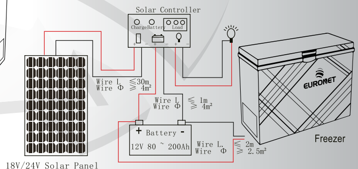
12V Solar Freezer System
