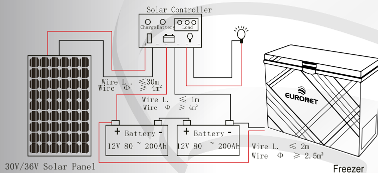
24V Solar Freezer System
